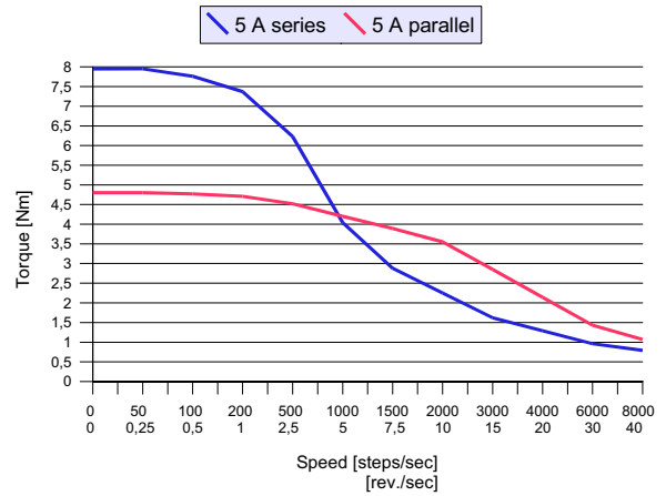
Torque/speed curves of SM41-5311 stepper motor with CD6410M module for 65 VDC
