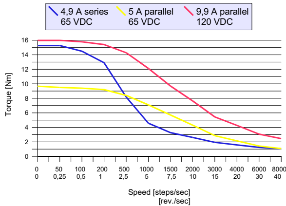
Torque/speed curves of SM42-4922 stepper motor with CD6410M module for 65 VDC and with CDZMP-Mini module for 120 VDC
