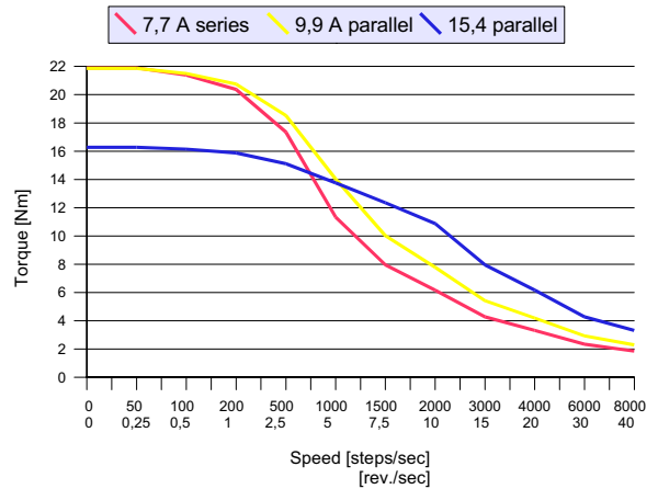
Torque/speed curves of SM43-7730 stepper motor (SM43-4930 for 9,9 A) with CDZMP-Mini module for 120 VDC
