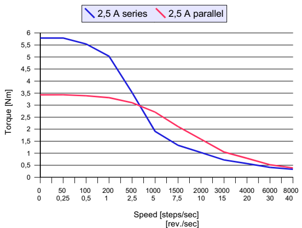
Torque/speed curves of SM32-2508 stepper motor with CD34M module for 48 VDC
